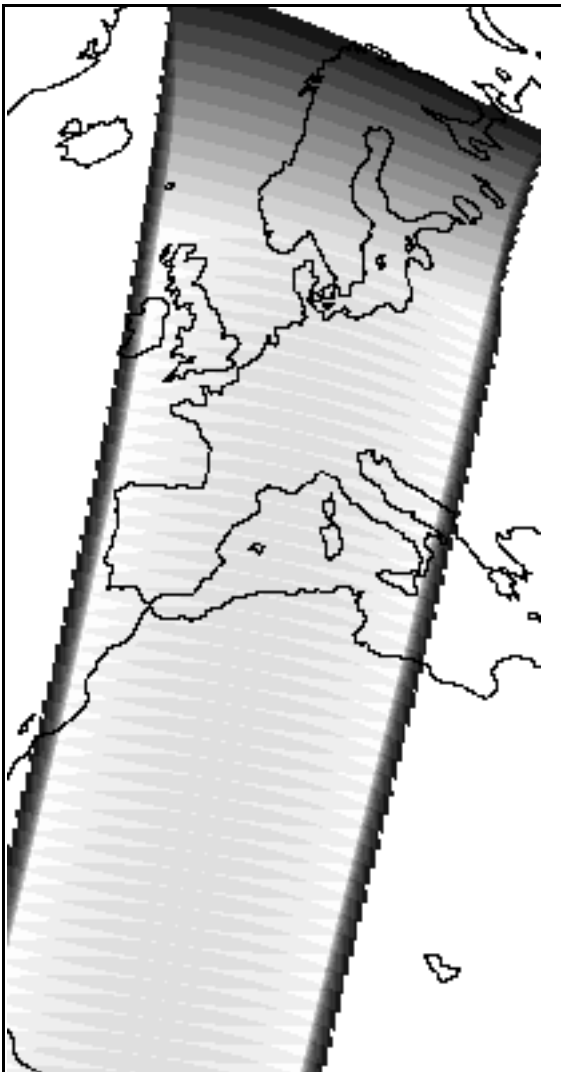
Fig. 3 : Number of viewing directions available for each surface pixel. Gray shades are from zero (Black) to fourteen (white). Twelve directions are available in the wide area around the satellite subtrack
